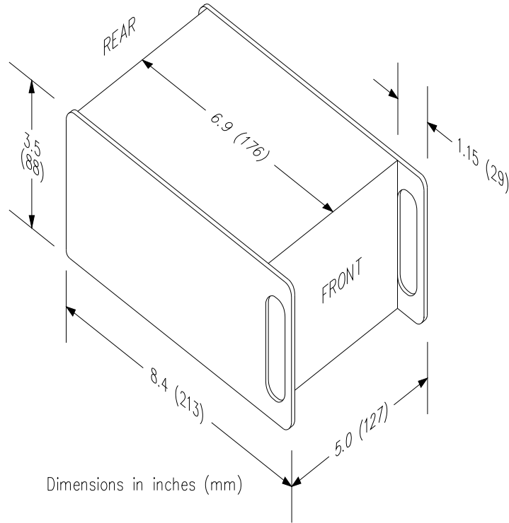
MODEL 781 SIGNAL CONDITIONING UNIT DIMENSIONS
